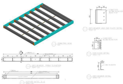
Shop Drawing
