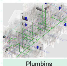
Plumbing
