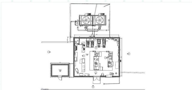
Mechanical Drawing
