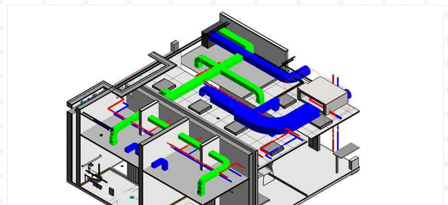
Clash Detection
