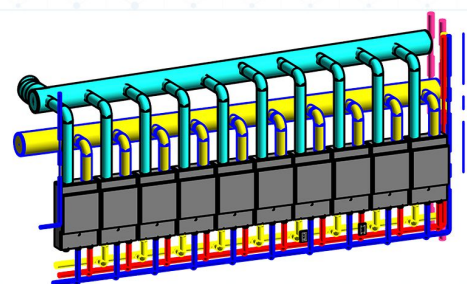
3D Model with LOD 350
