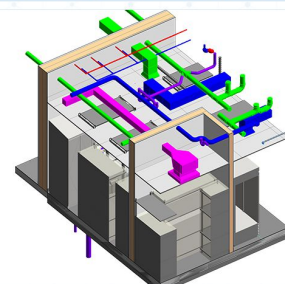
Clash Detection
