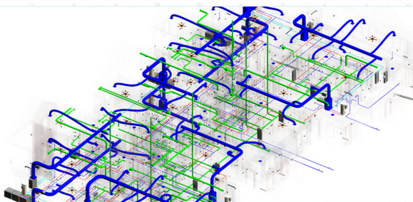
3D Model
