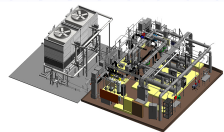
3D Model with LOD 400
