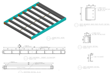
Shop Drawing
