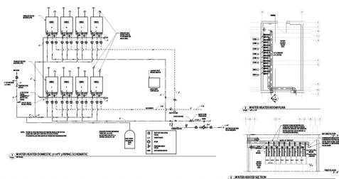
Plumbing Drawing
